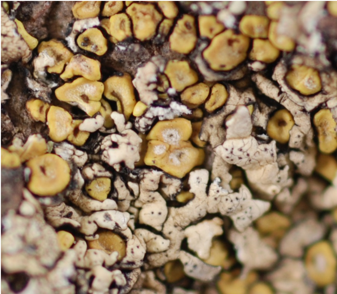
Figure 1. Holotype of Acarospora stictica.
